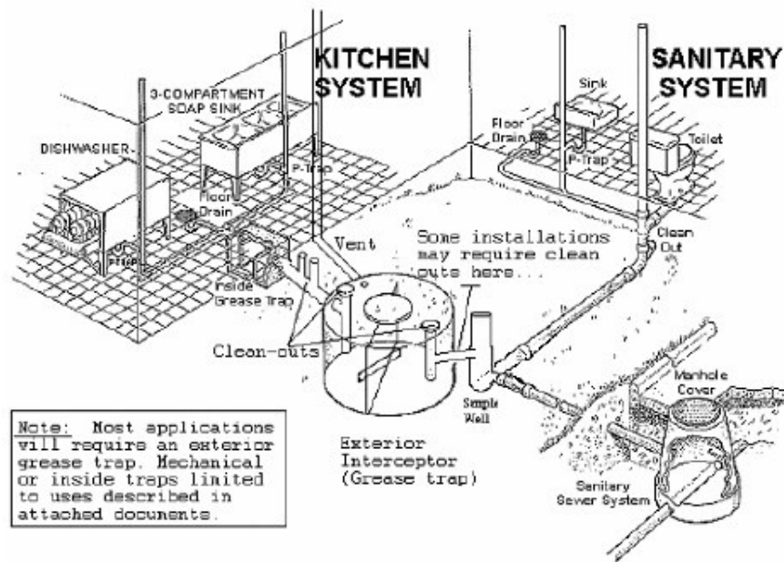
Figure 1, Typical plumbing layout
